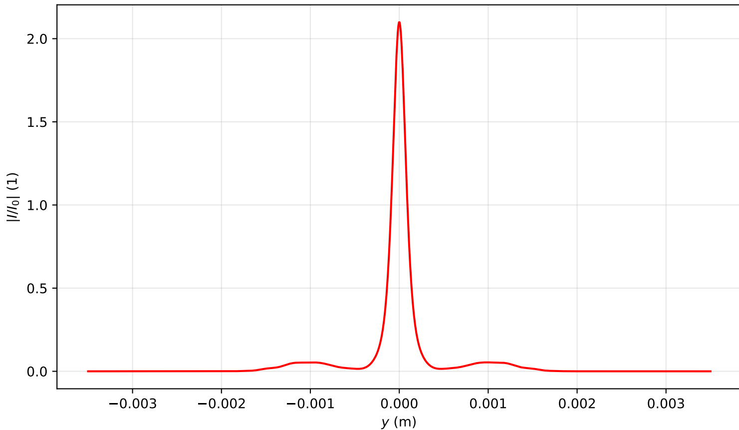
Intensity profile I(x = 0, y, z = 2.627)/I_0 , P_{in}=8.0P_{cr} , artificial time
